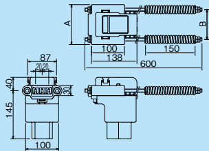
Drawing shows a 3P end tension insulator.
